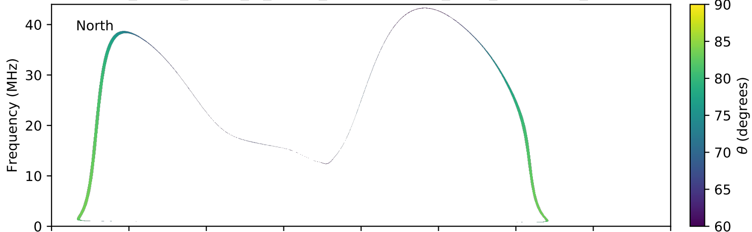
expres_earth_jupiter_io_jrm09_lossc-wid1deg_3kev_20040719_v11.cdf
