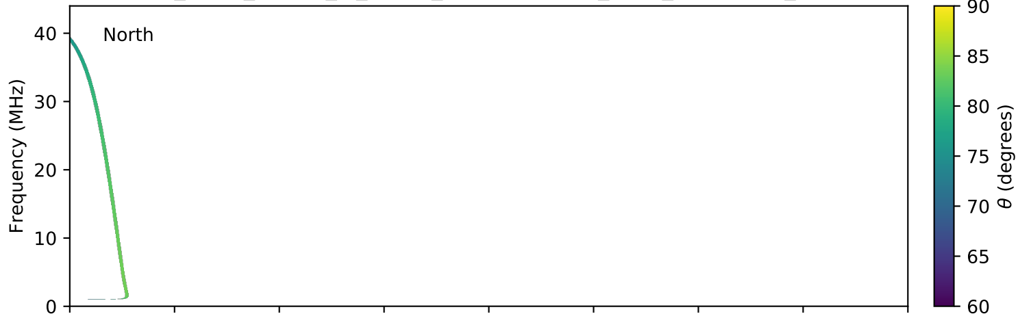
expres_earth_jupiter_io_jrm09_lossc-wid1deg_3kev_20040718_v11.cdf
