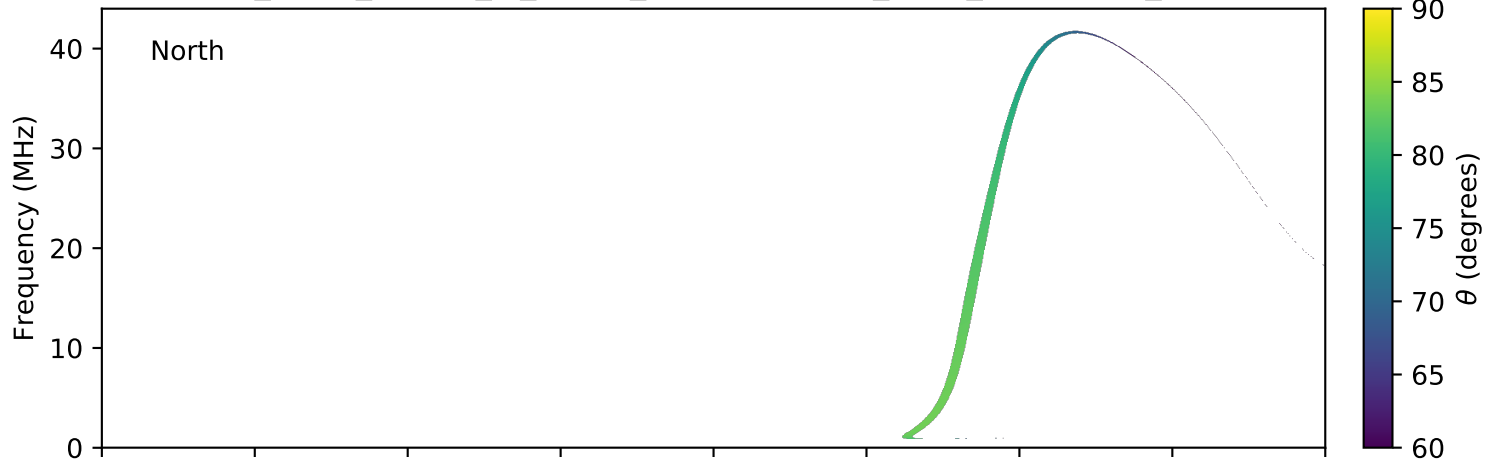
expres_earth_jupiter_io_jrm09_lossc-wid1deg_3kev_20040715_v11.cdf
