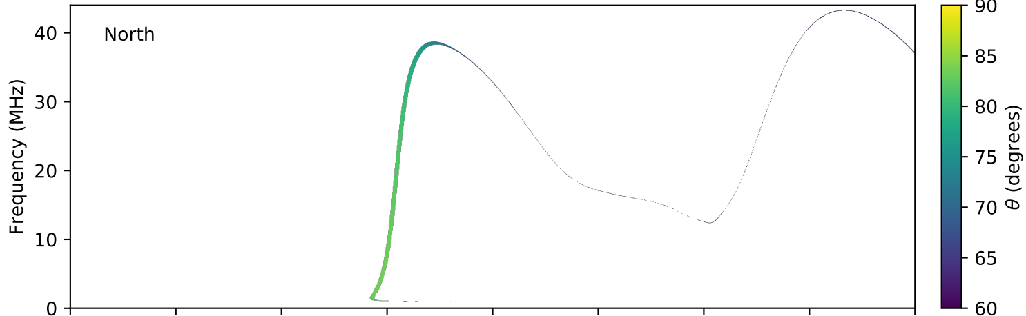
expres_earth_jupiter_io_jrm09_lossc-wid1deg_3kev_20040710_v11.cdf
