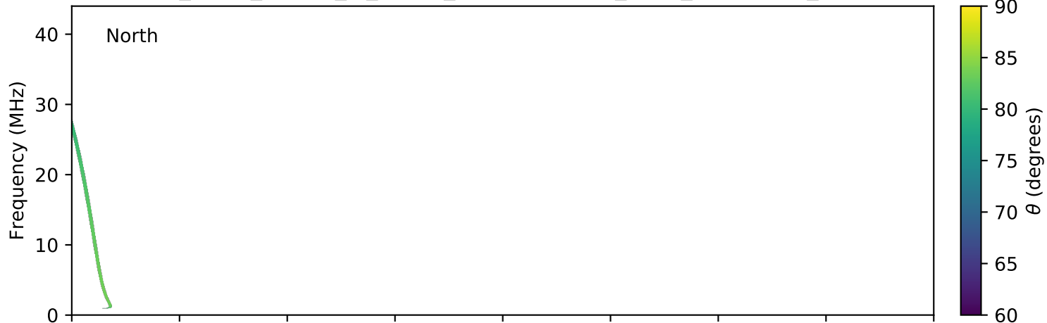
expres_earth_jupiter_io_jrm09_lossc-wid1deg_3kev_20040704_v11.cdf
