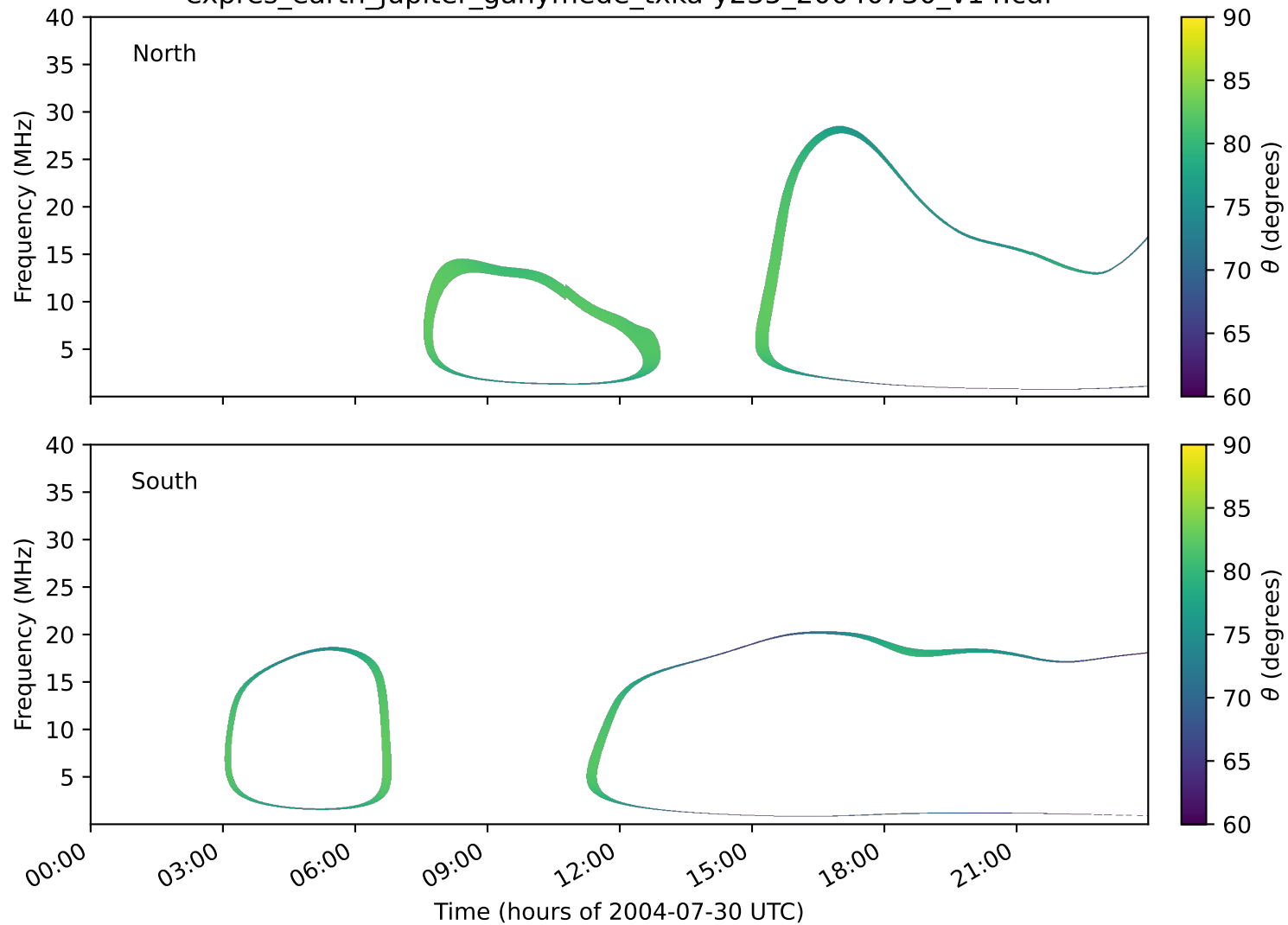
expres_earth_jupiter_ganymede_txka-y235_20040730_v14.cdf
