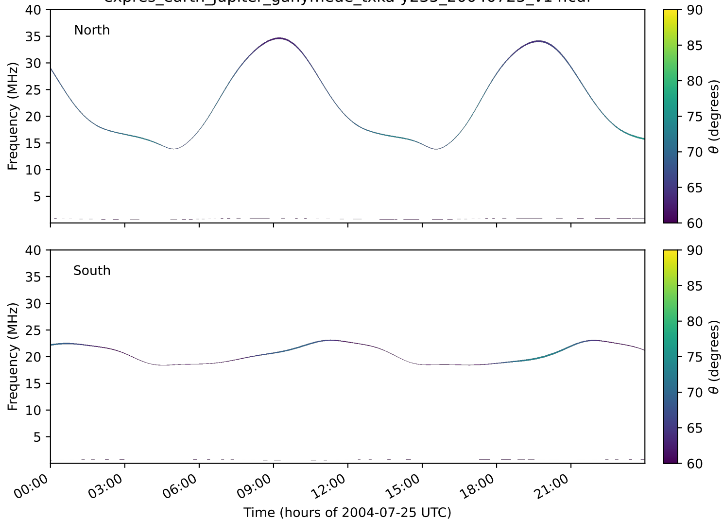
expres_earth_jupiter_ganymede_txka-y235_20040725_v14.cdf
