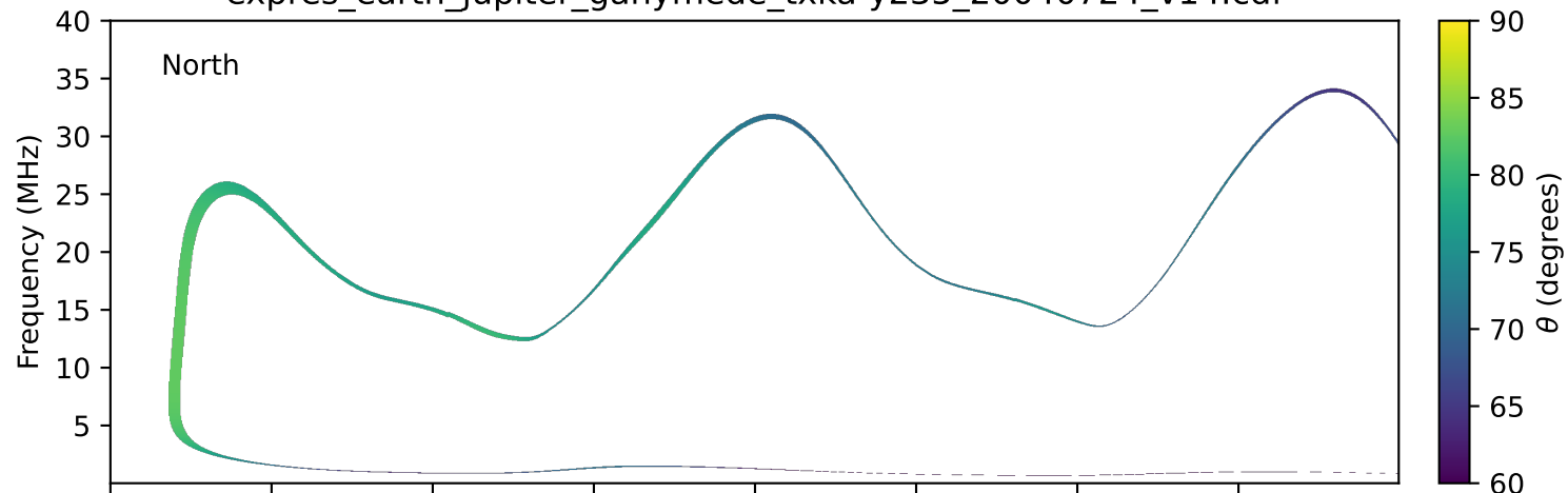
expres_earth_jupiter_ganymede_txka-y235_20040724_v14.cdf
