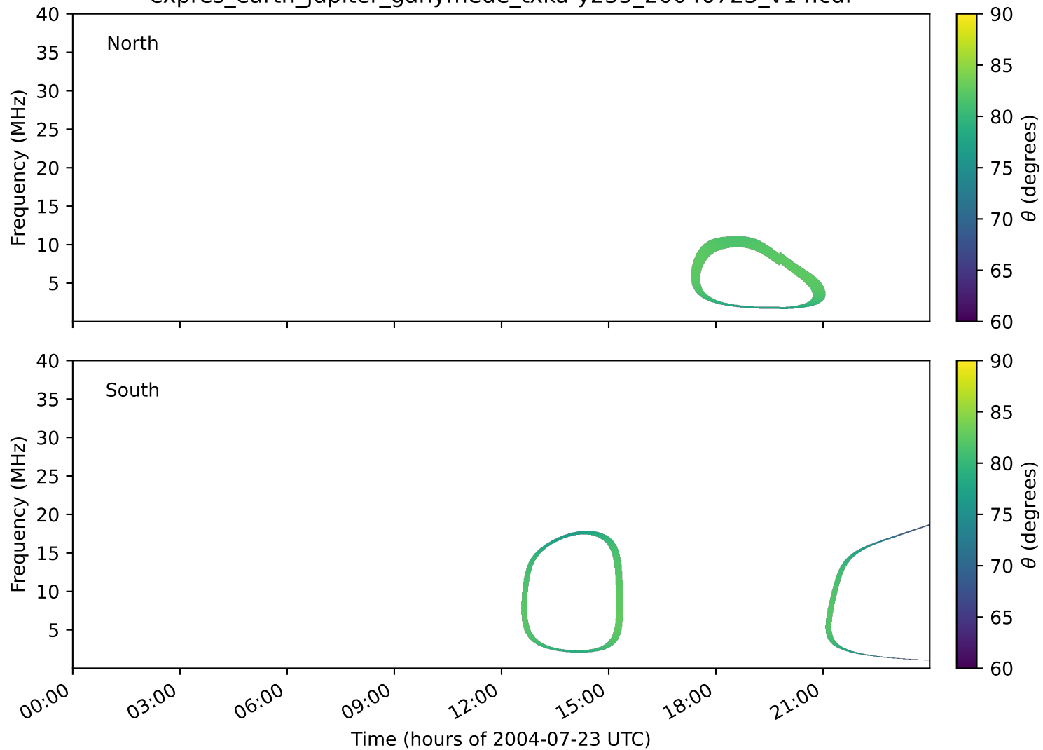
expres_earth_jupiter_ganymede_txka-y235_20040723_v14.cdf
