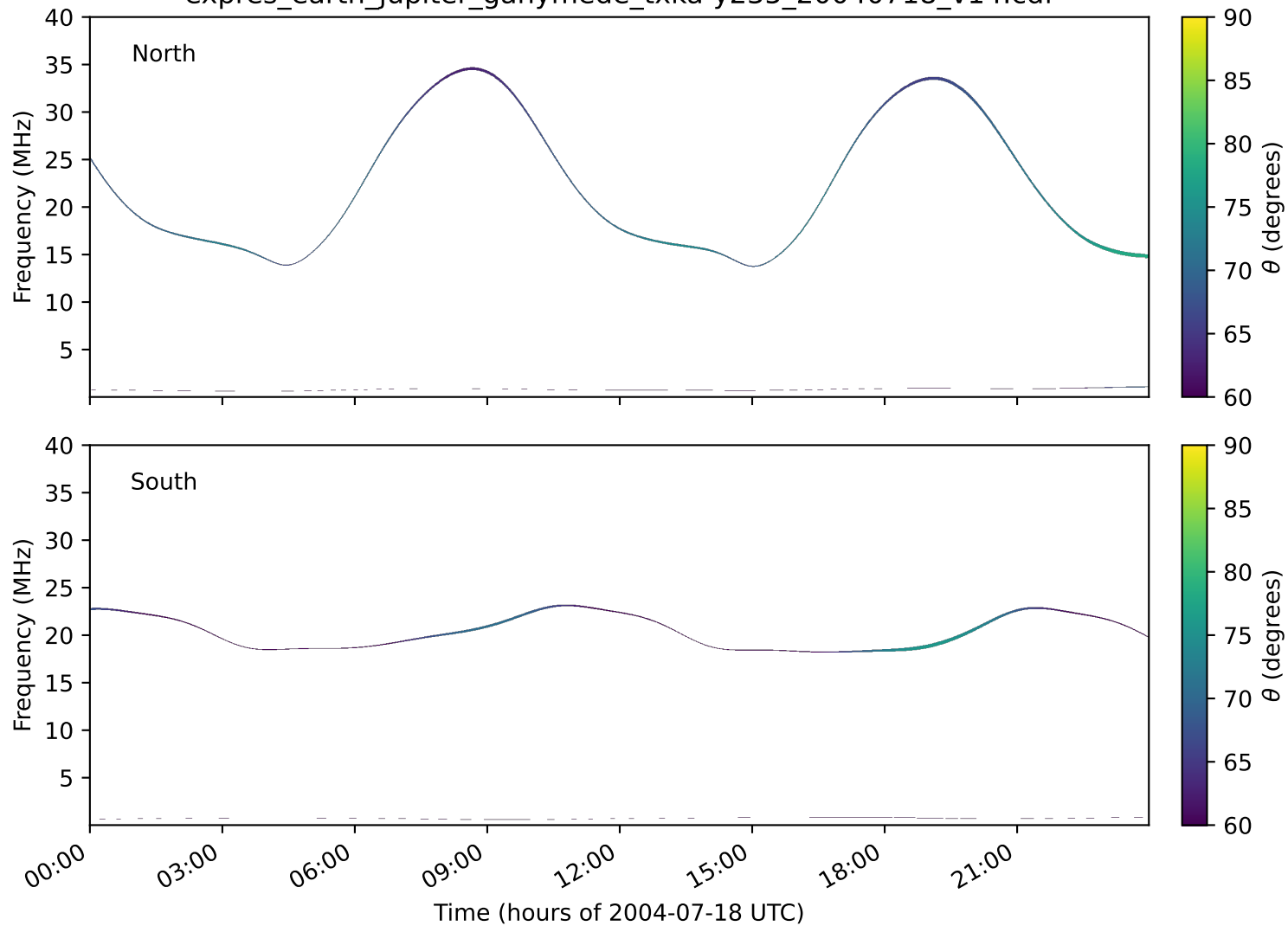
expres_earth_jupiter_ganymede_txka-y235_20040718_v14.cdf
