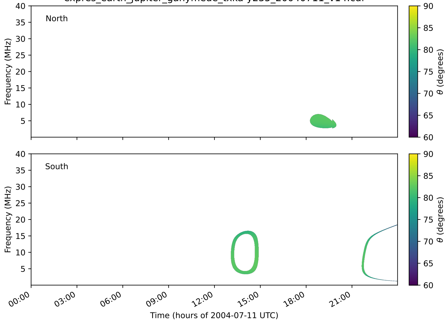
expres_earth_jupiter_ganymede_txka-y235_20040711_v14.cdf
