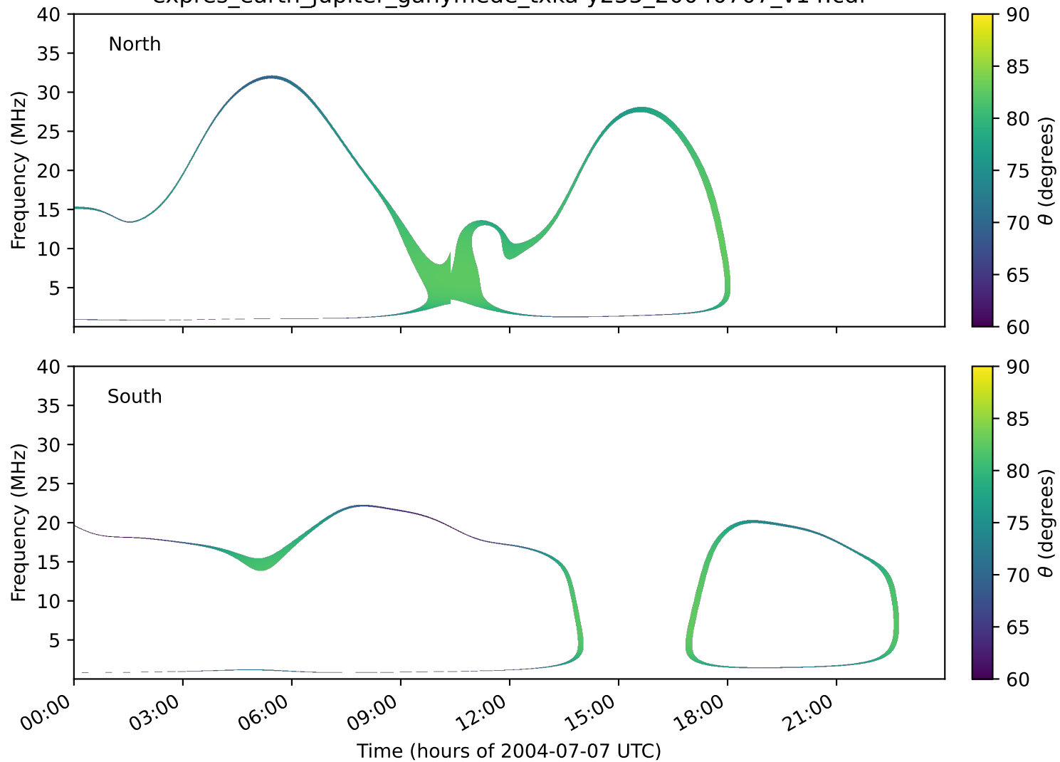
expres_earth_jupiter_ganymede_txka-y235_20040707_v14.cdf
