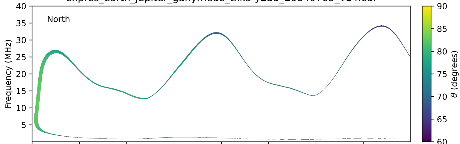
expres_earth_jupiter_ganymede_txka-y235_20040705_v14.cdf
