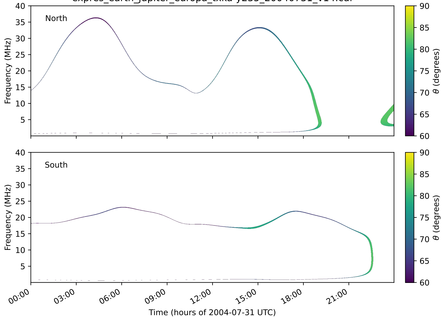
expres_earth_jupiter_europa_txka-y235_20040731_v14.cdf
