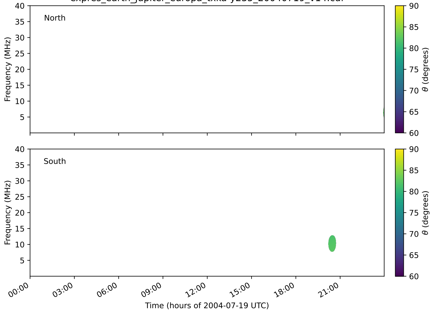
expres_earth_jupiter_europa_txka-y235_20040719_v14.cdf
