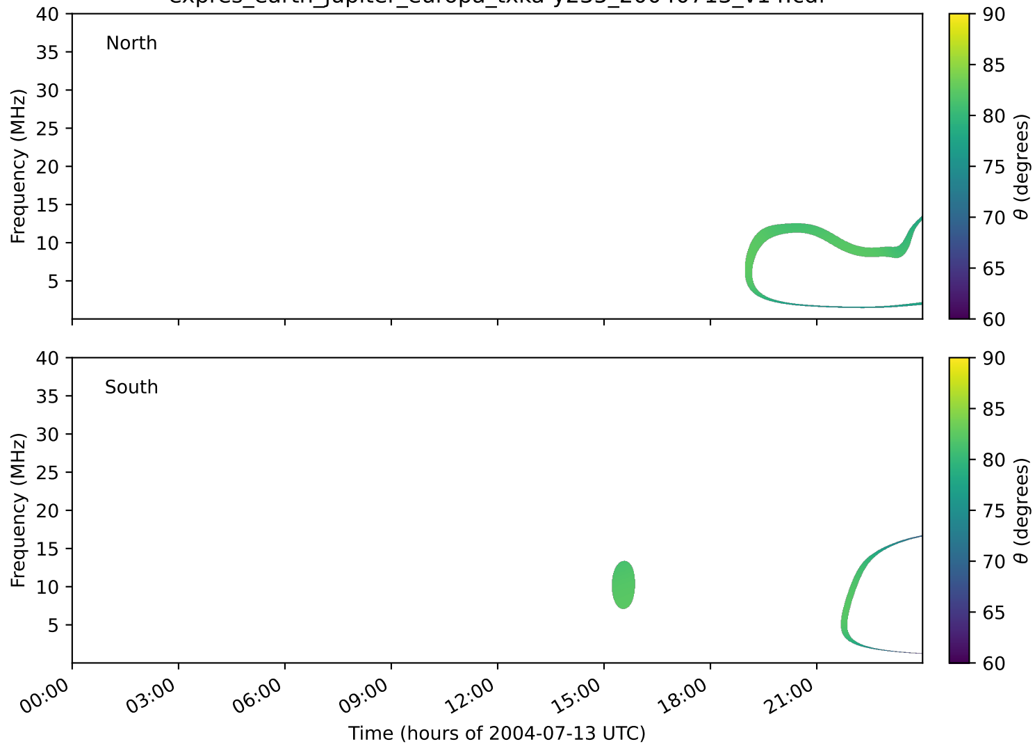
expres_earth_jupiter_europa_txka-y235_20040713_v14.cdf
