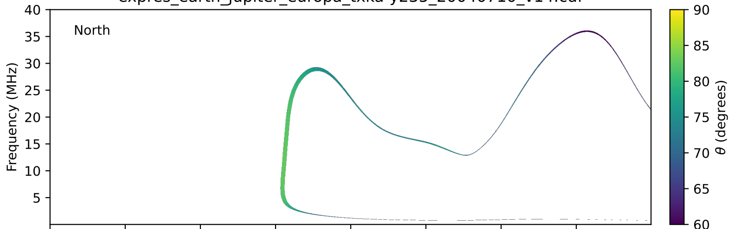
expres_earth_jupiter_europa_txka-y235_20040710_v14.cdf
