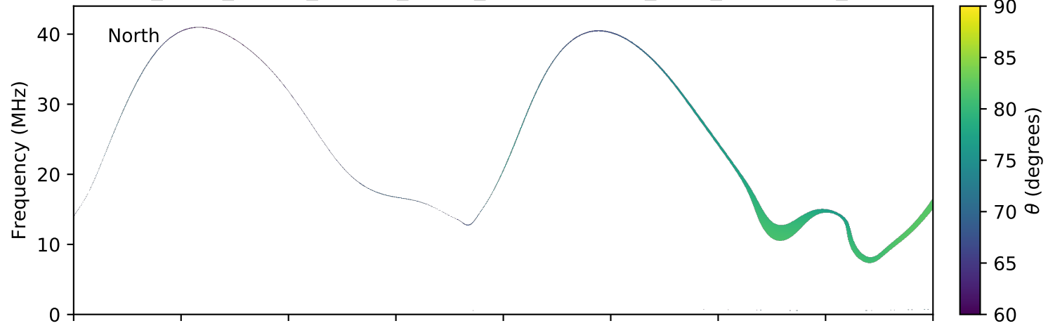
expres_earth_jupiter_europa_jrm09_lossc-wid1deg_3kev_20040731_v11.cdf
