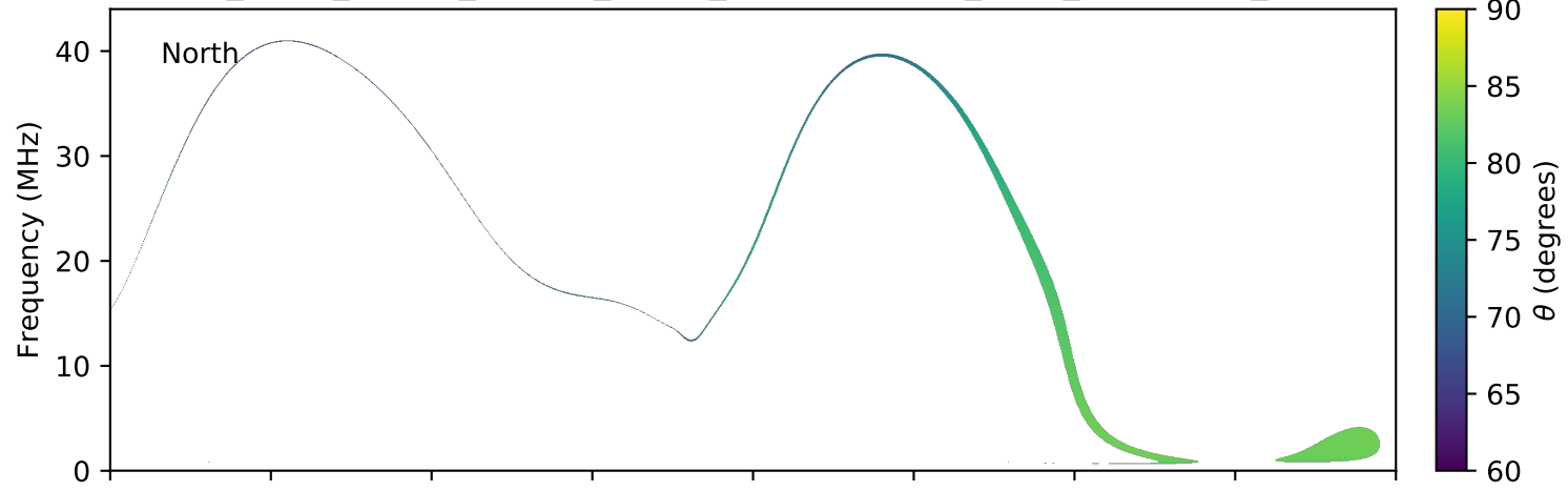
expres_earth_jupiter_europa_jrm09_lossc-wid1deg_3kev_20040728_v11.cdf
