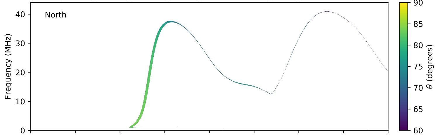
expres_earth_jupiter_europa_jrm09_lossc-wid1deg_3kev_20040727_v11.cdf
