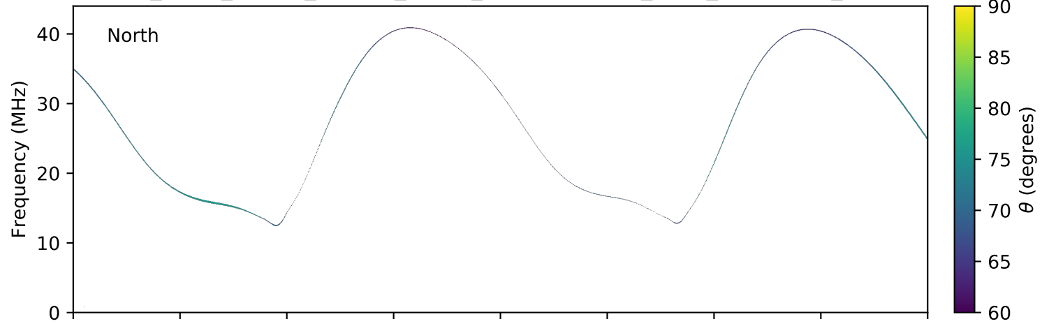
expres_earth_jupiter_europa_jrm09_lossc-wid1deg_3kev_20040724_v11.cdf
