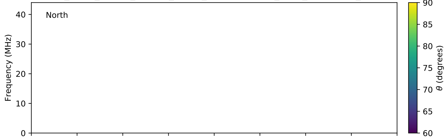
expres_earth_jupiter_europa_jrm09_lossc-wid1deg_3kev_20040719_v11.cdf
