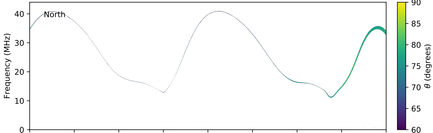
expres_earth_jupiter_europa_jrm09_lossc-wid1deg_3kev_20040717_v11.cdf
