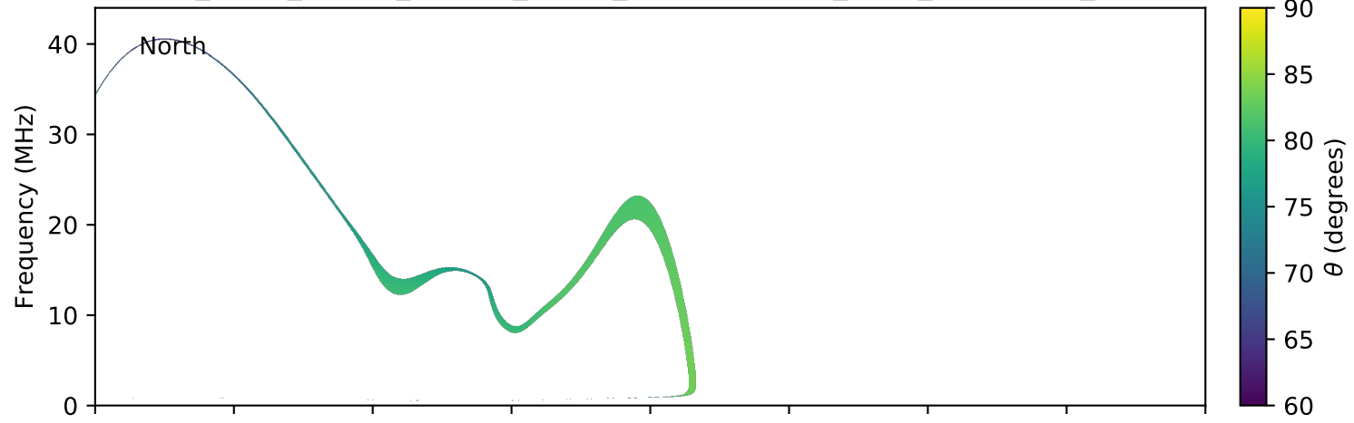
expres_earth_jupiter_europa_jrm09_lossc-wid1deg_3kev_20040715_v11.cdf
