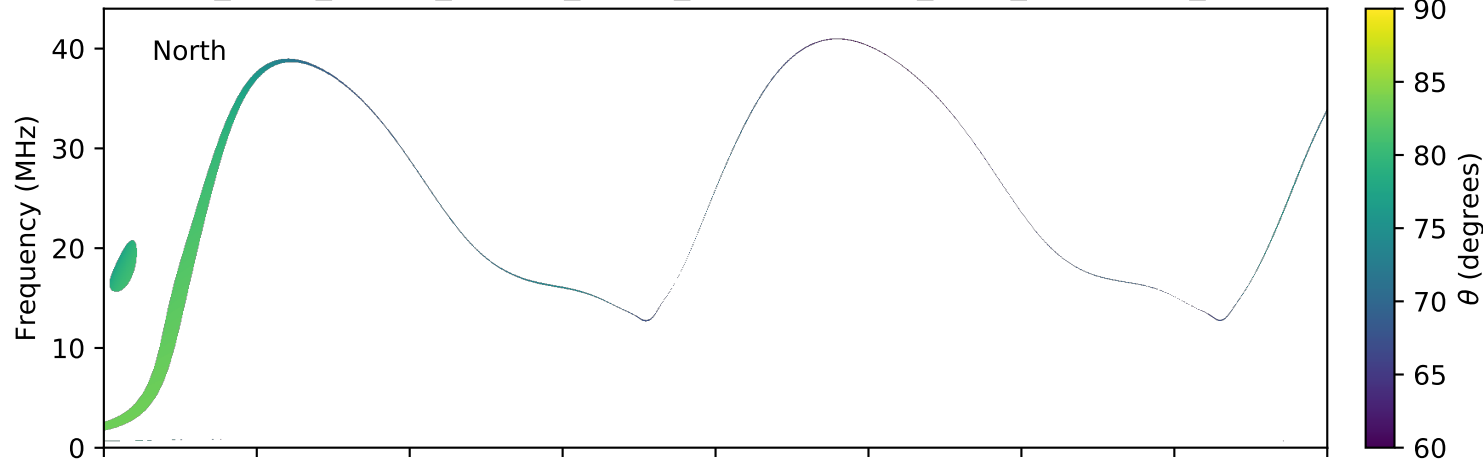
expres_earth_jupiter_europa_jrm09_lossc-wid1deg_3kev_20040714_v11.cdf
