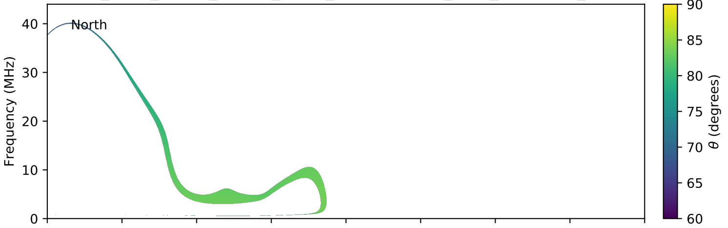
expres_earth_jupiter_europa_jrm09_lossc-wid1deg_3kev_20040708_v11.cdf
