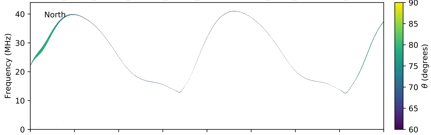
expres_earth_jupiter_europa_jrm09_lossc-wid1deg_3kev_20040707_v11.cdf
