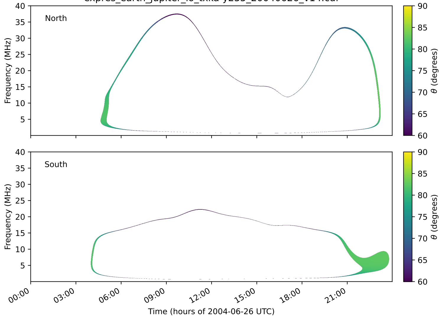
expres_earth_jupiter_io_txka-y235_20040626_v14.cdf
