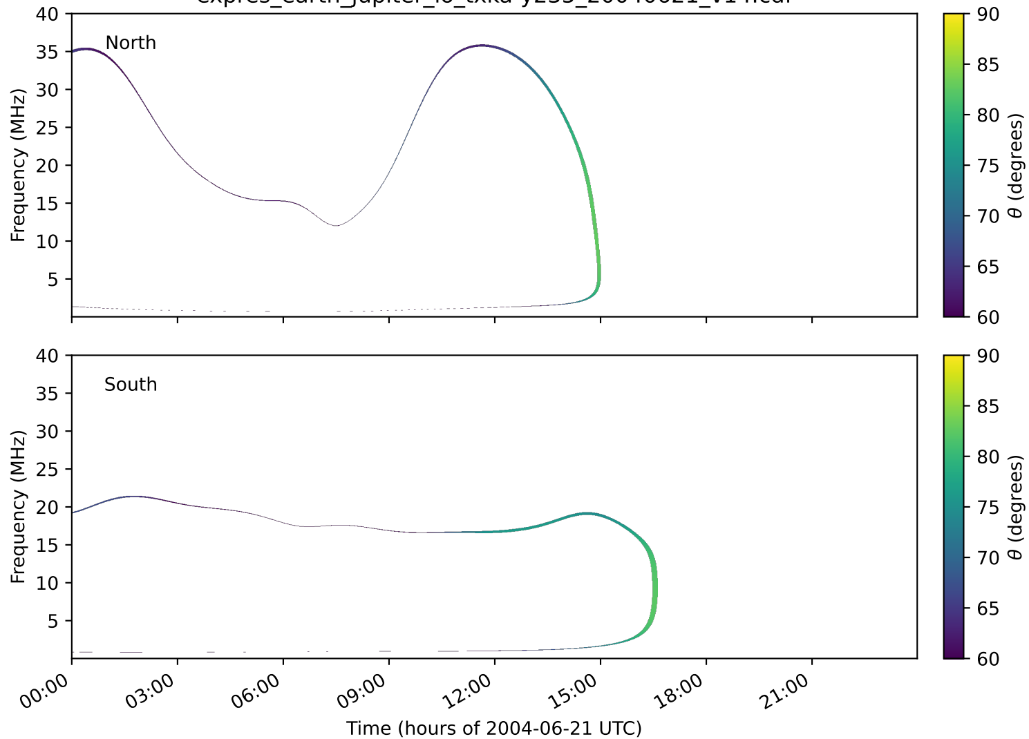
expres_earth_jupiter_io_txka-y235_20040621_v14.cdf
