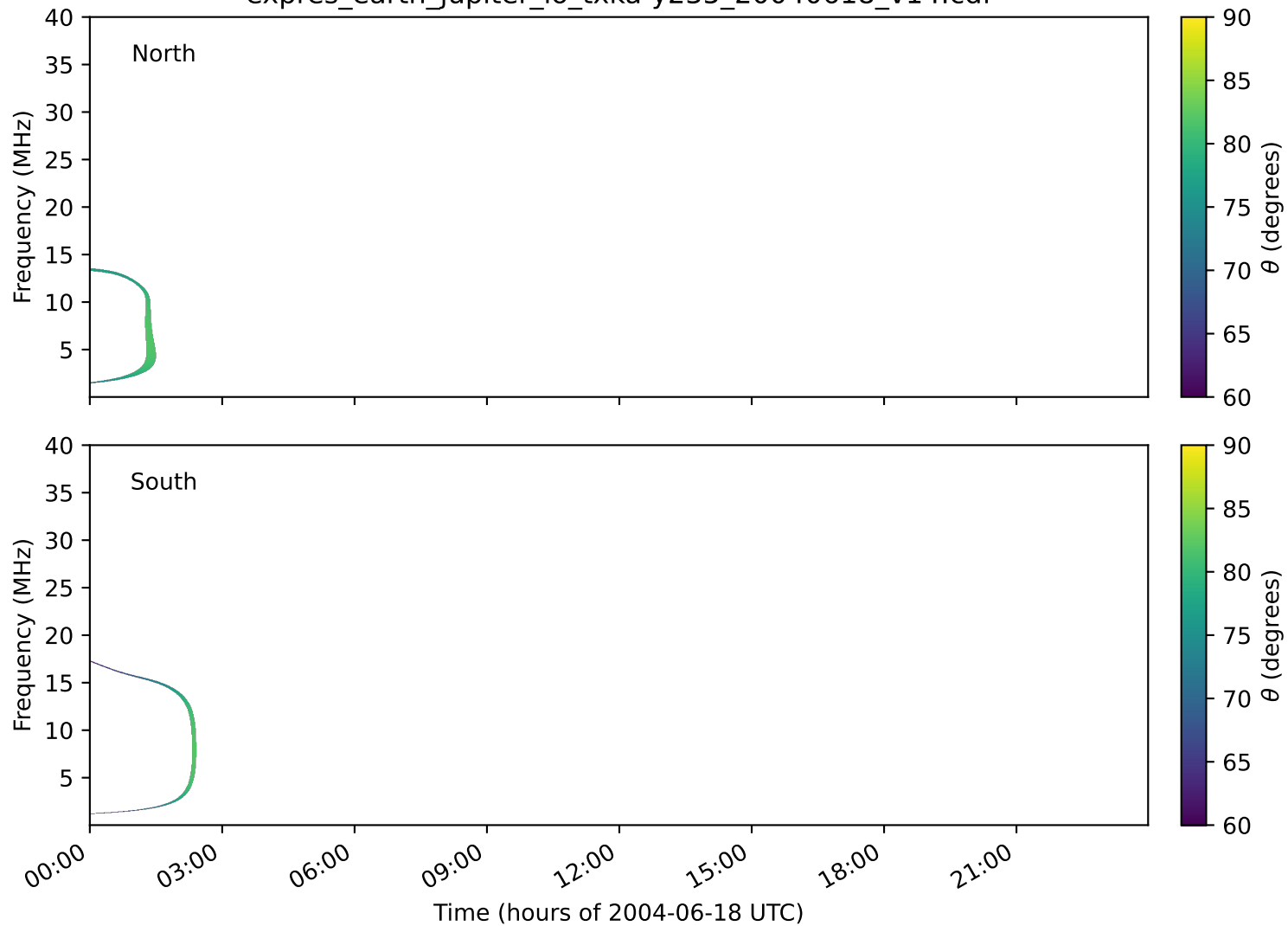
expres_earth_jupiter_io_txka-y235_20040618_v14.cdf
