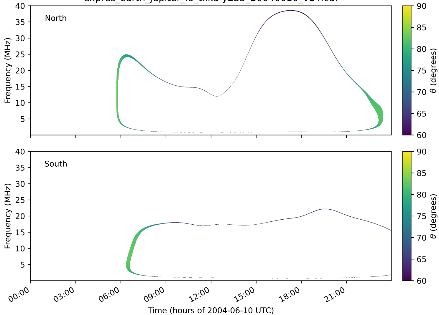
expres_earth_jupiter_io_txka-y235_20040610_v14.cdf
