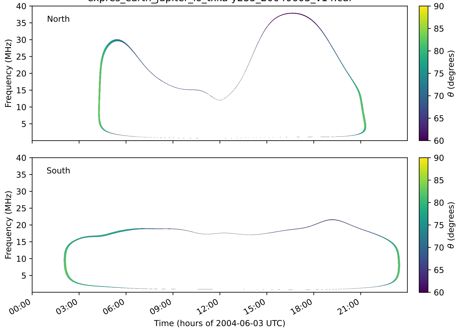
expres_earth_jupiter_io_txka-y235_20040603_v14.cdf
