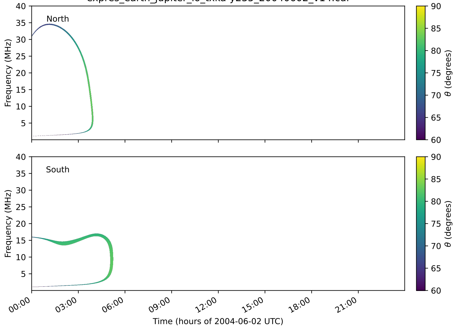
expres_earth_jupiter_io_txka-y235_20040602_v14.cdf
