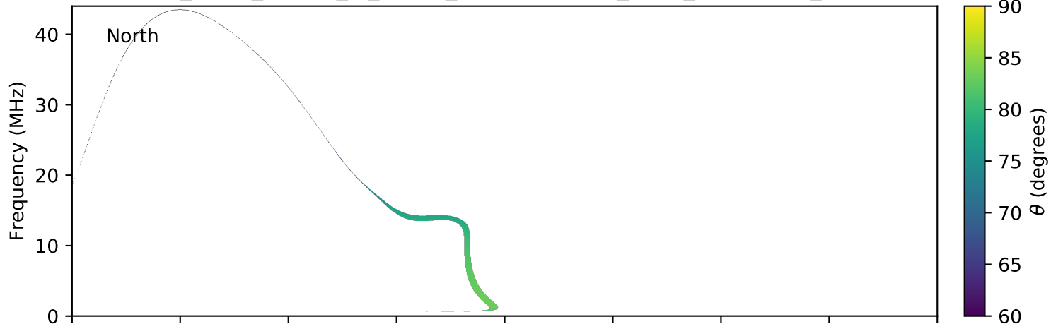
expres_earth_jupiter_io_jrm09_lossc-wid1deg_3kev_20040630_v11.cdf
