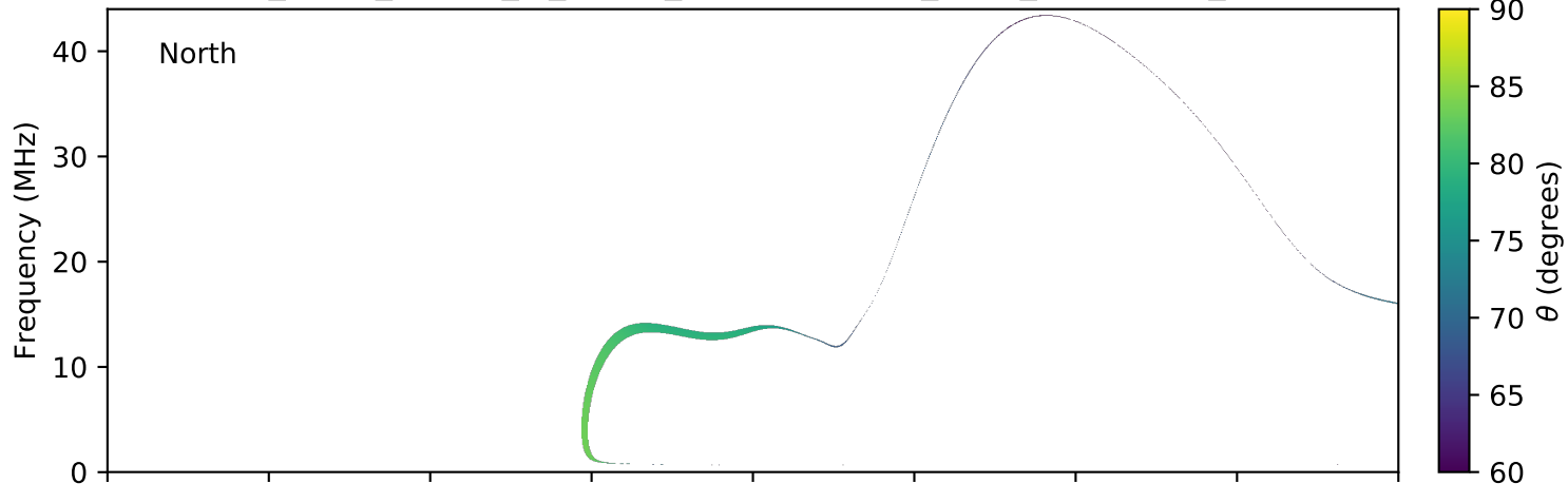
expres_earth_jupiter_io_jrm09_lossc-wid1deg_3kev_20040624_v11.cdf
