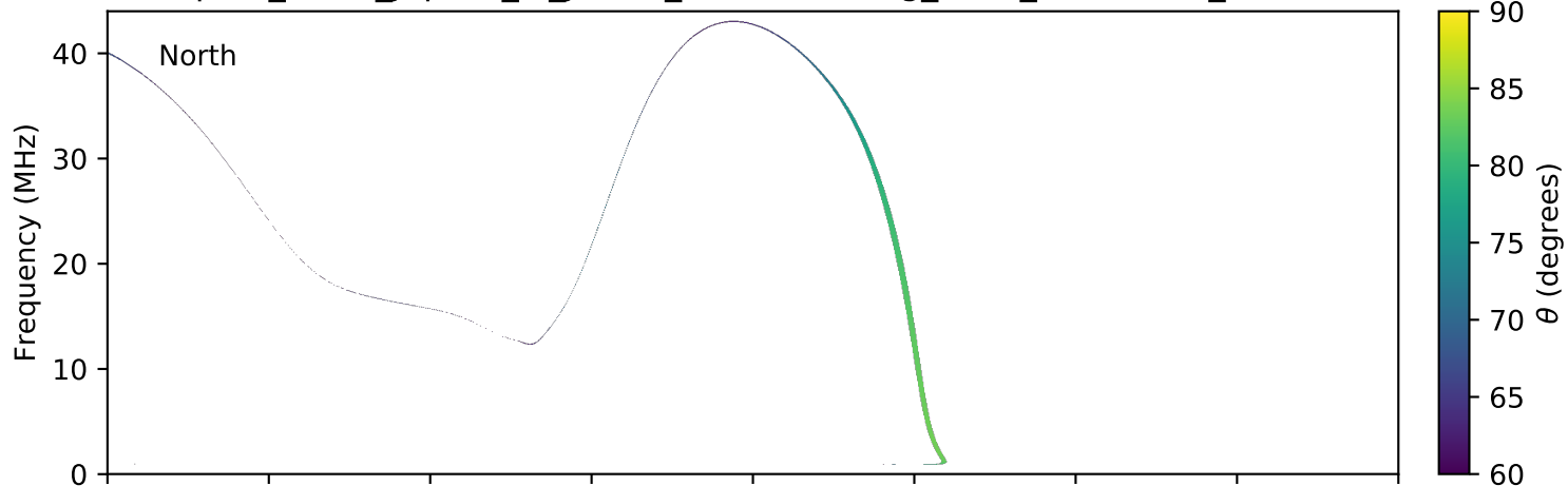
expres_earth_jupiter_io_jrm09_lossc-wid1deg_3kev_20040621_v11.cdf
