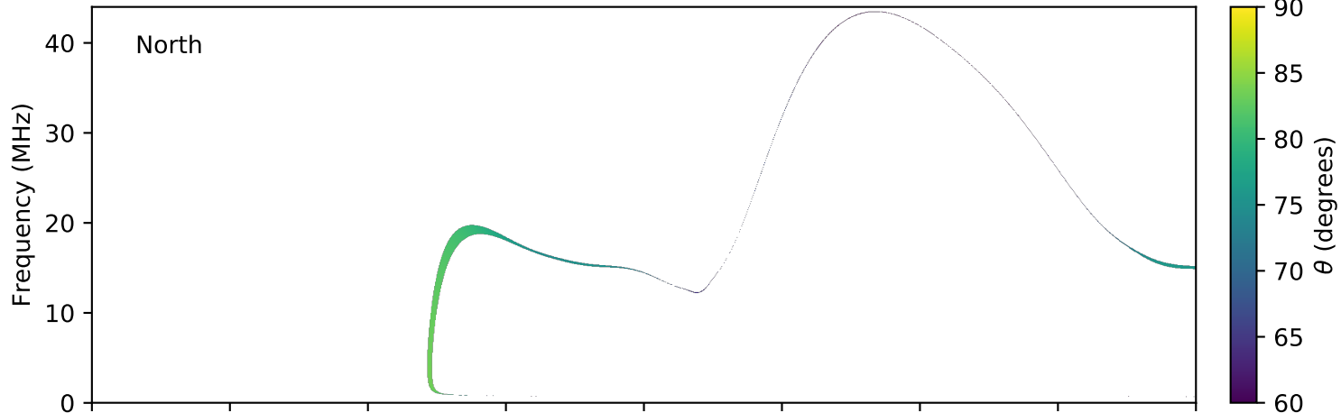
expres_earth_jupiter_io_jrm09_lossc-wid1deg_3kev_20040617_v11.cdf
