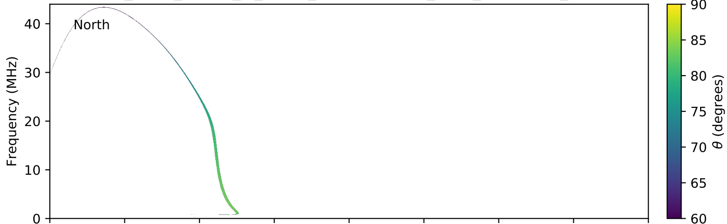
expres_earth_jupiter_io_jrm09_lossc-wid1deg_3kev_20040616_v11.cdf
