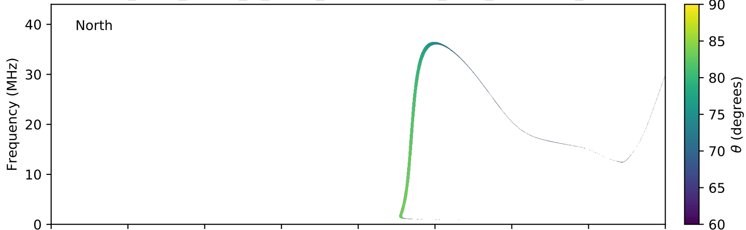
expres_earth_jupiter_io_jrm09_lossc-wid1deg_3kev_20040615_v11.cdf
