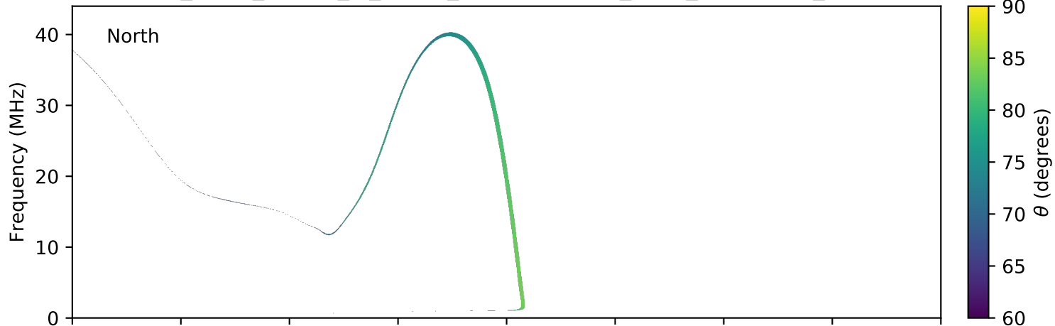
expres_earth_jupiter_io_jrm09_lossc-wid1deg_3kev_20040607_v11.cdf
