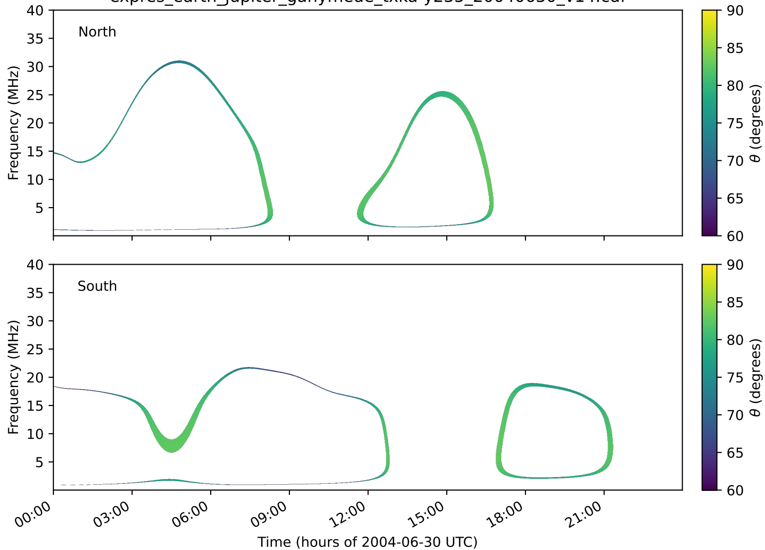
expres_earth_jupiter_ganymede_txka-y235_20040630_v14.cdf
