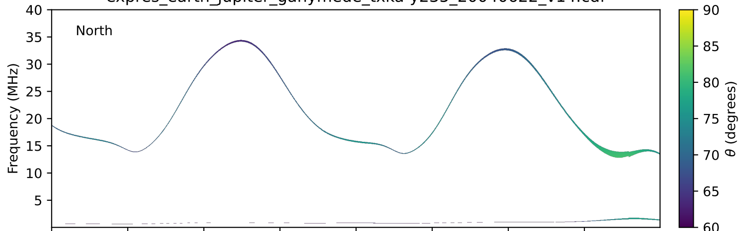
expres_earth_jupiter_ganymede_txka-y235_20040622_v14.cdf
