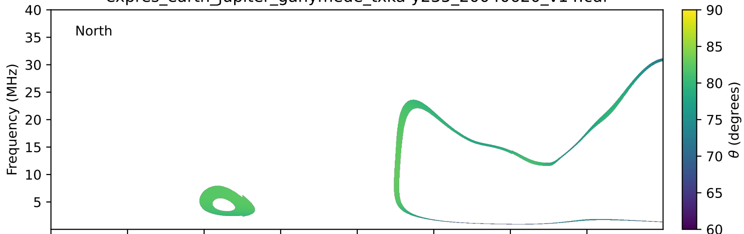
expres_earth_jupiter_ganymede_txka-y235_20040620_v14.cdf
