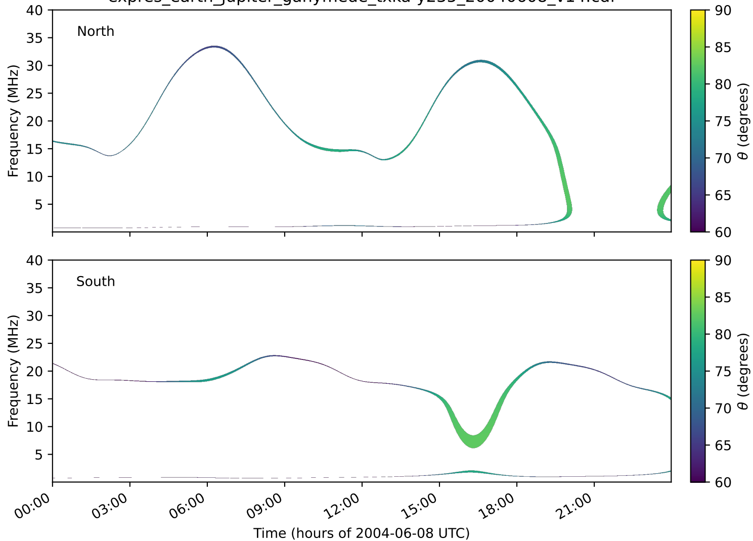
expres_earth_jupiter_ganymede_txka-y235_20040608_v14.cdf
