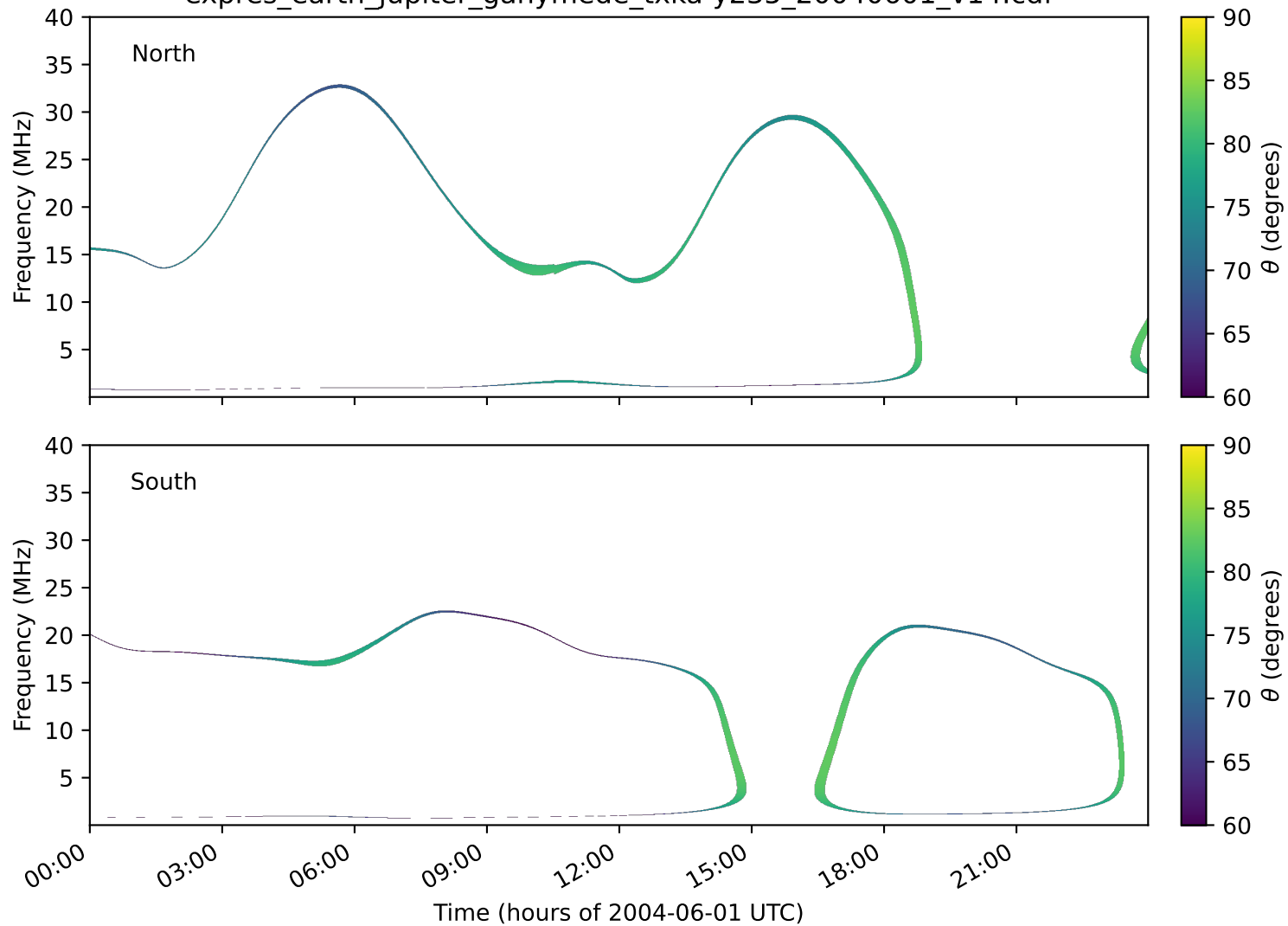
expres_earth_jupiter_ganymede_txka-y235_20040601_v14.cdf
