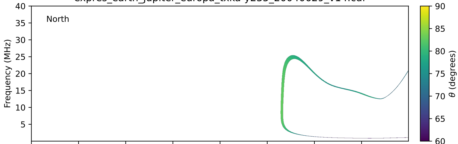
expres_earth_jupiter_europa_txka-y235_20040629_v14.cdf
