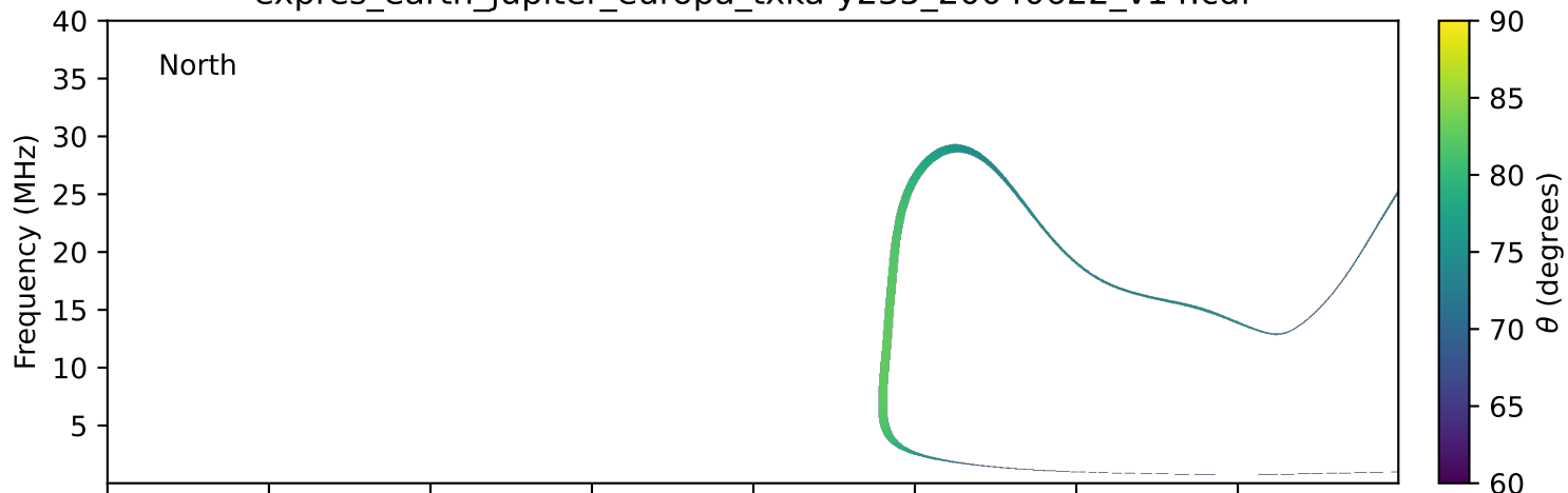
expres_earth_jupiter_europa_txka-y235_20040622_v14.cdf
