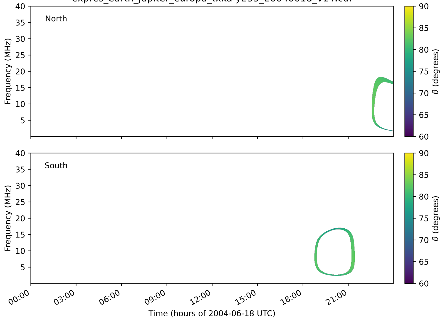
expres_earth_jupiter_europa_txka-y235_20040618_v14.cdf
