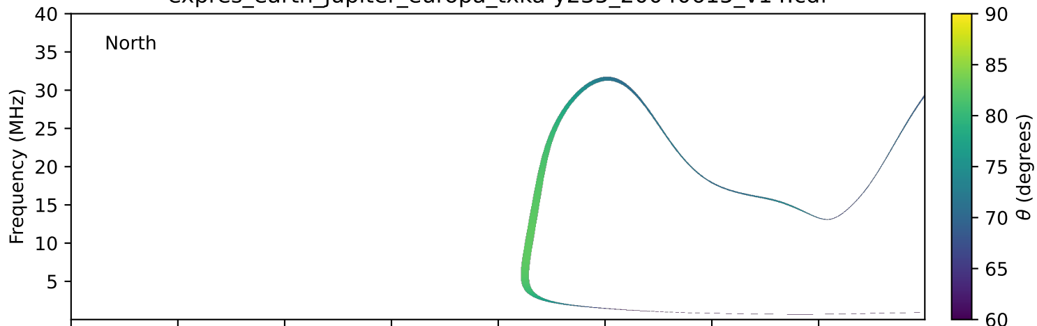
expres_earth_jupiter_europa_txka-y235_20040615_v14.cdf
