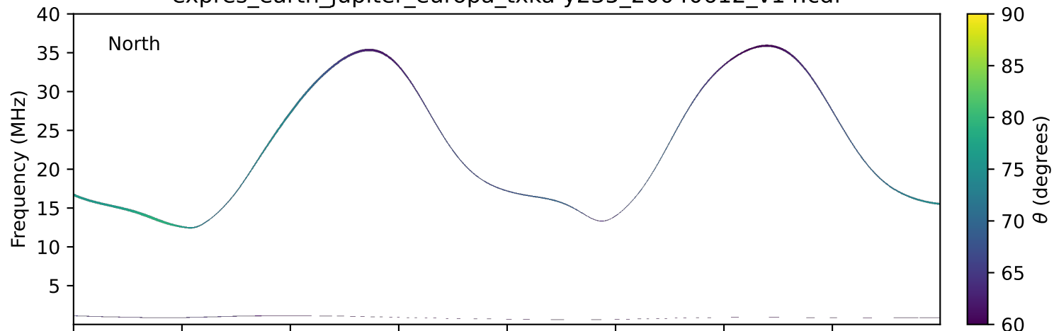
expres_earth_jupiter_europa_txka-y235_20040612_v14.cdf
